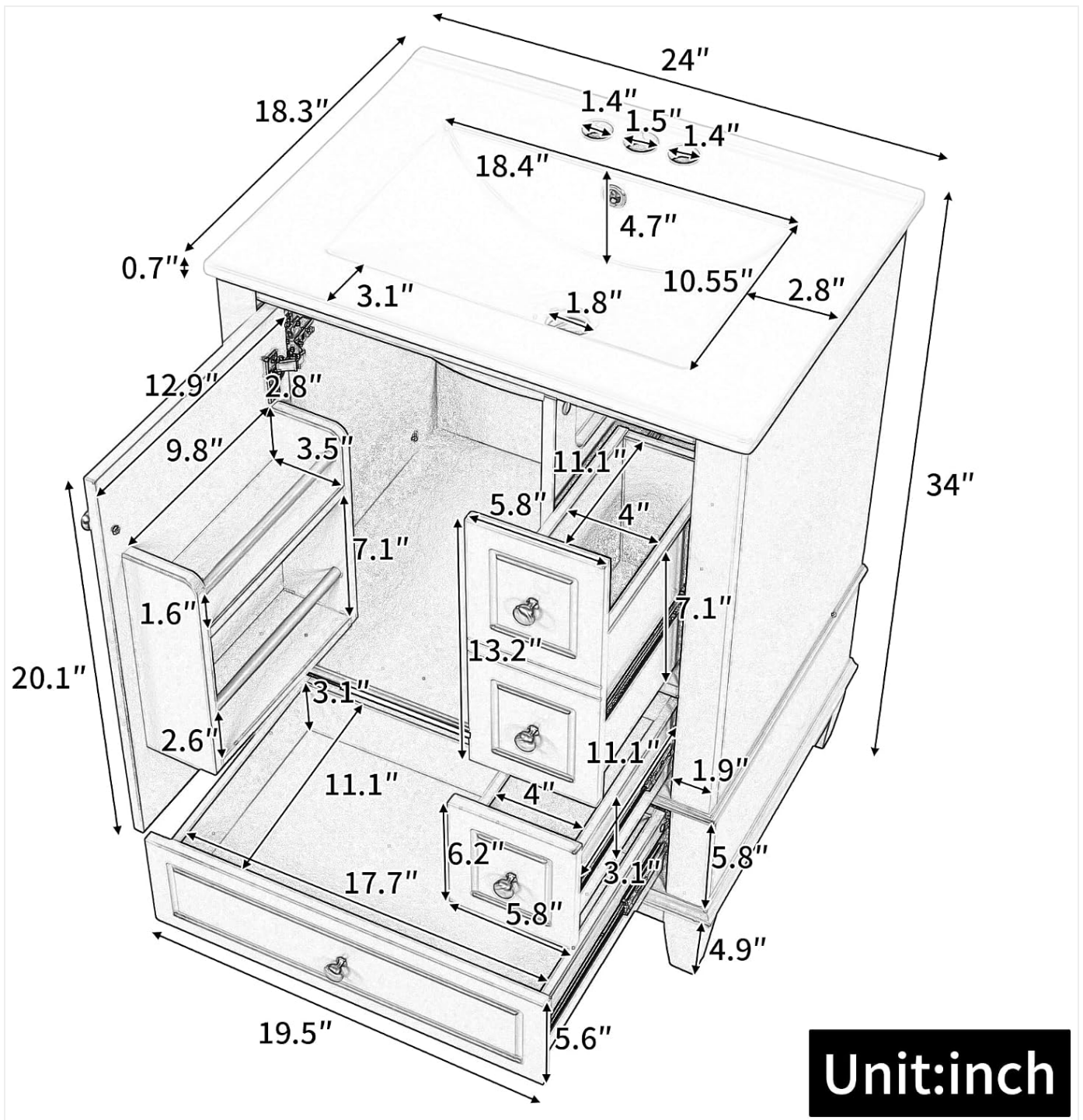
Figure 2: Product Dimensions (Unit: Inch)
