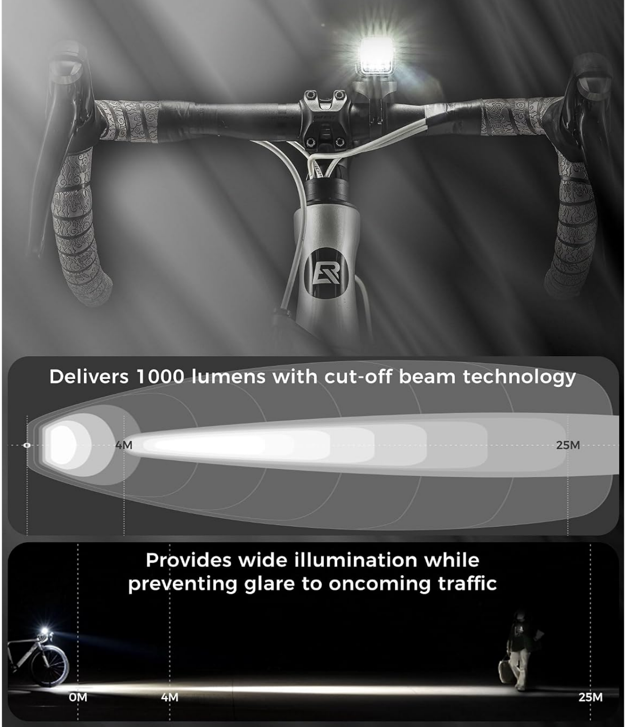
Figure 4.2: This diagram highlights the anti-glare design of the RHL1000, which delivers 1000 lumens with cut-off beam technology. This feature provides wide illumination for the rider while preventing glare for oncoming traffic.
