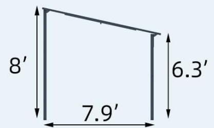
Image: Dimensional diagram of the AECOJOY 14' x 8' Hard Top Lean-to Gazebo.
