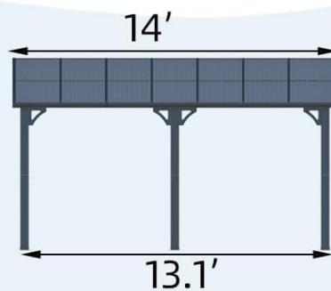
Image: Dimensional diagram of the AECOJOY 14' x 8' Hard Top Lean-to Gazebo.
