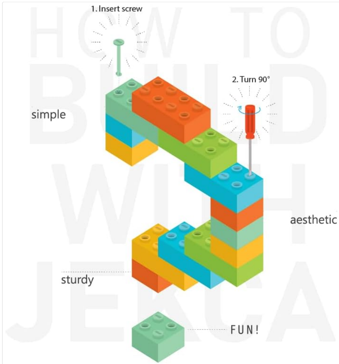
Figure 1: JEKCA Interlocking System. This diagram illustrates the two-step process: 1. Insert the pin into the brick. 2. Turn the pin 90 degrees using the pin driver to lock the bricks securely. This method ensures the model's stability without glue.
