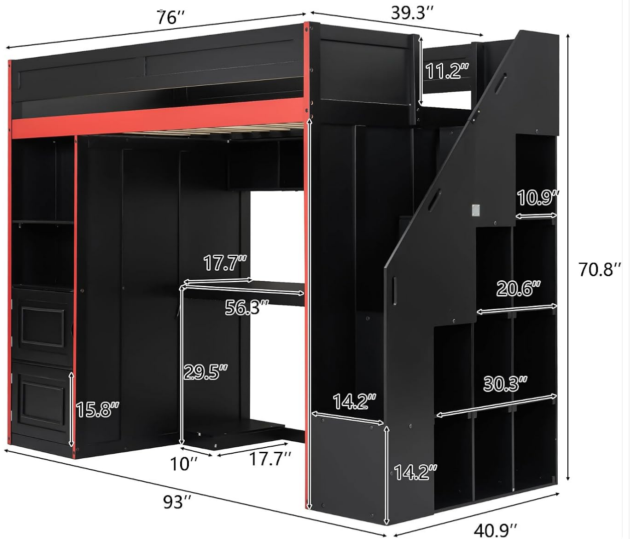
Image: Dimensional diagram of the loft bed, showing all key measurements in inches.
