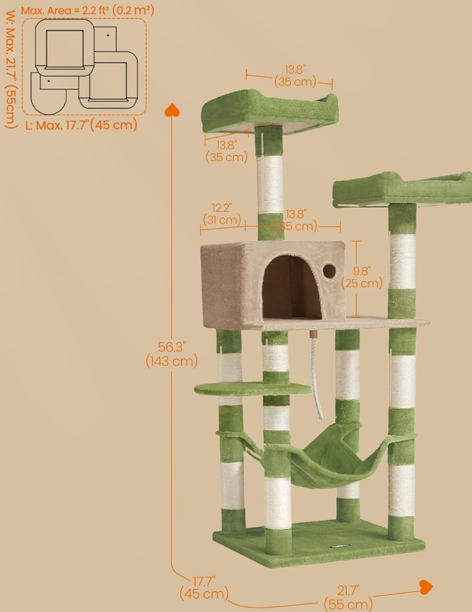
Figure 6: Detailed dimensions and recommended cat weight for the cat tree.
