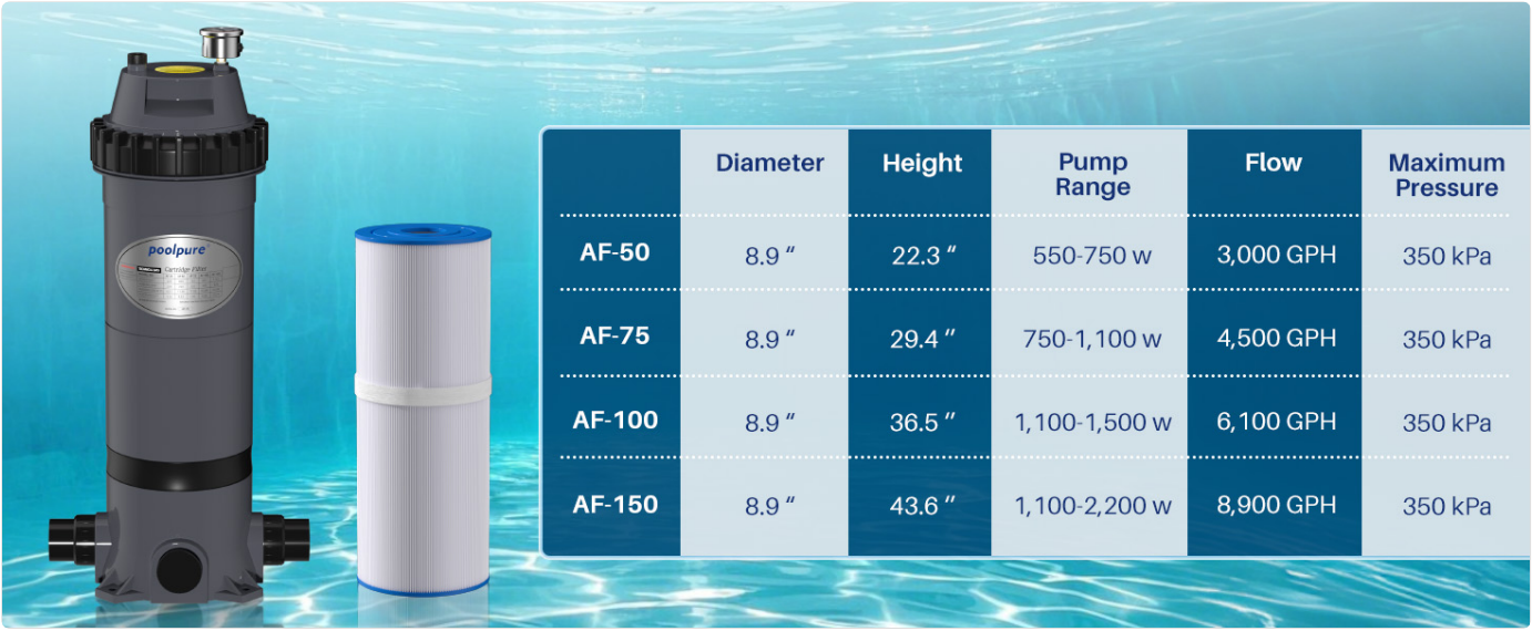
Figure 4: POOLPURE Cartridge Filter Model Comparison
