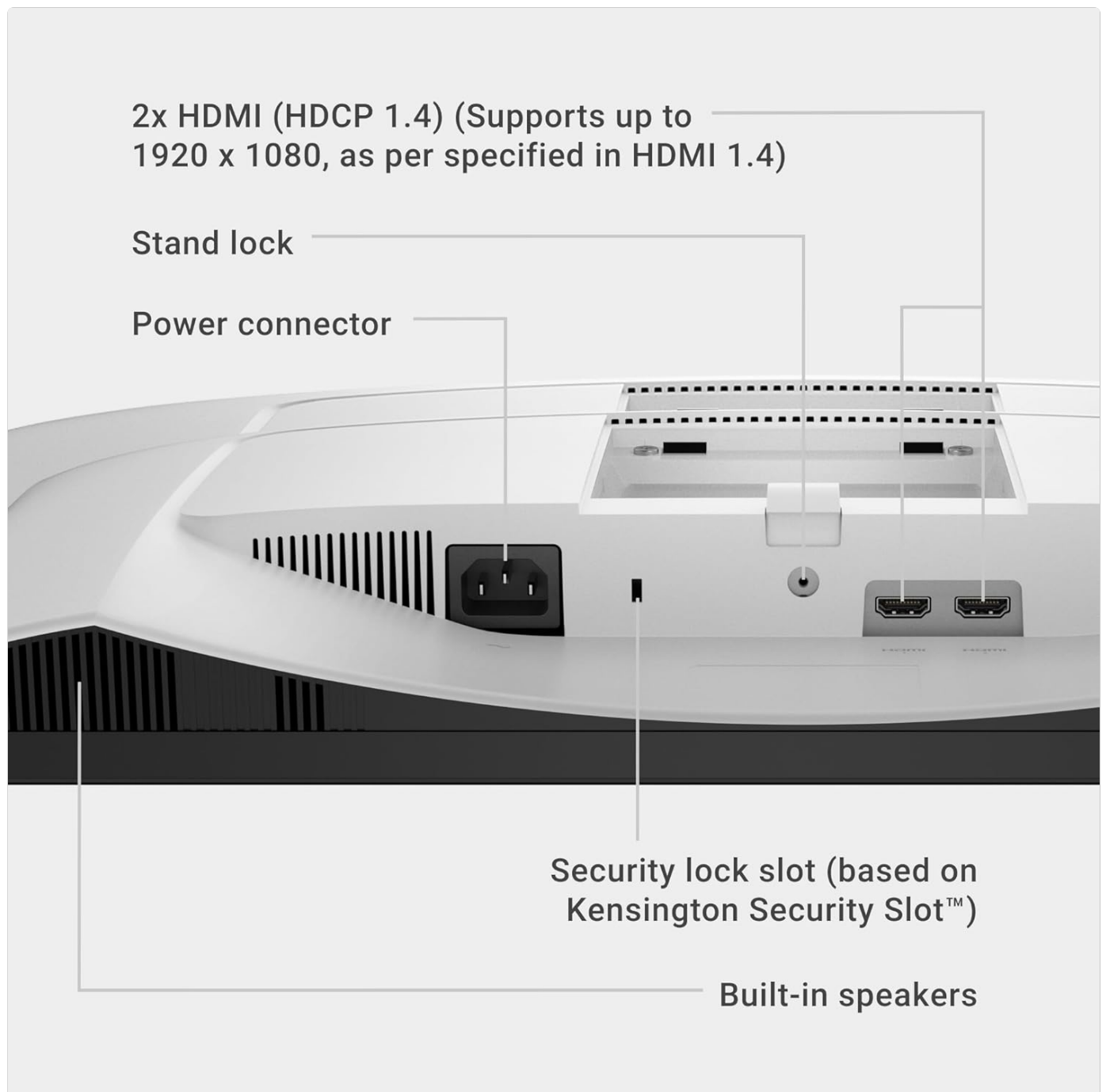
Figure 3.2: Rear view of the Dell S2425HSM monitor showing HDMI ports, power connector, and security lock slot.
