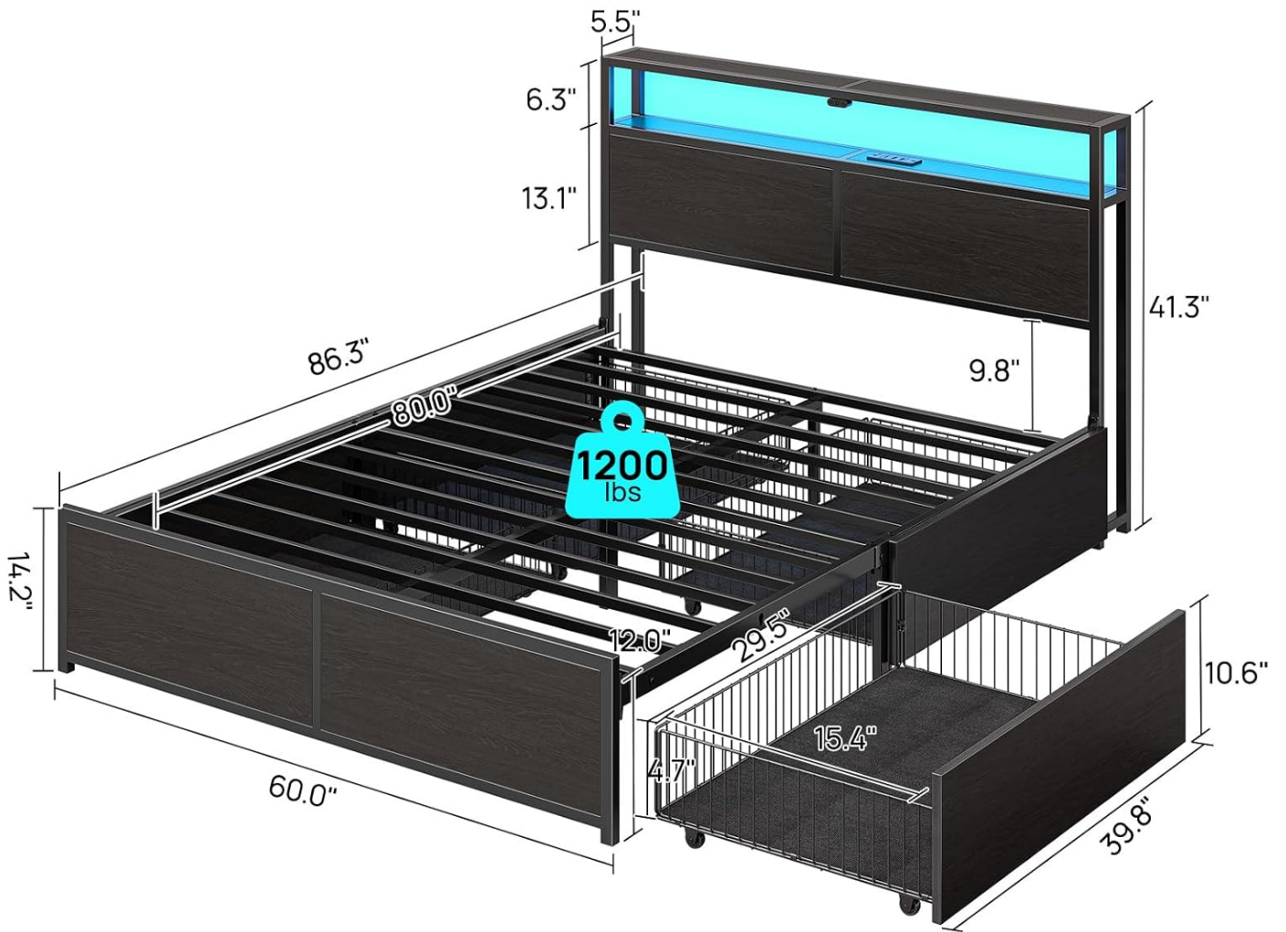
Figure 8: Product dimensions of the Queen Bed Frame.
