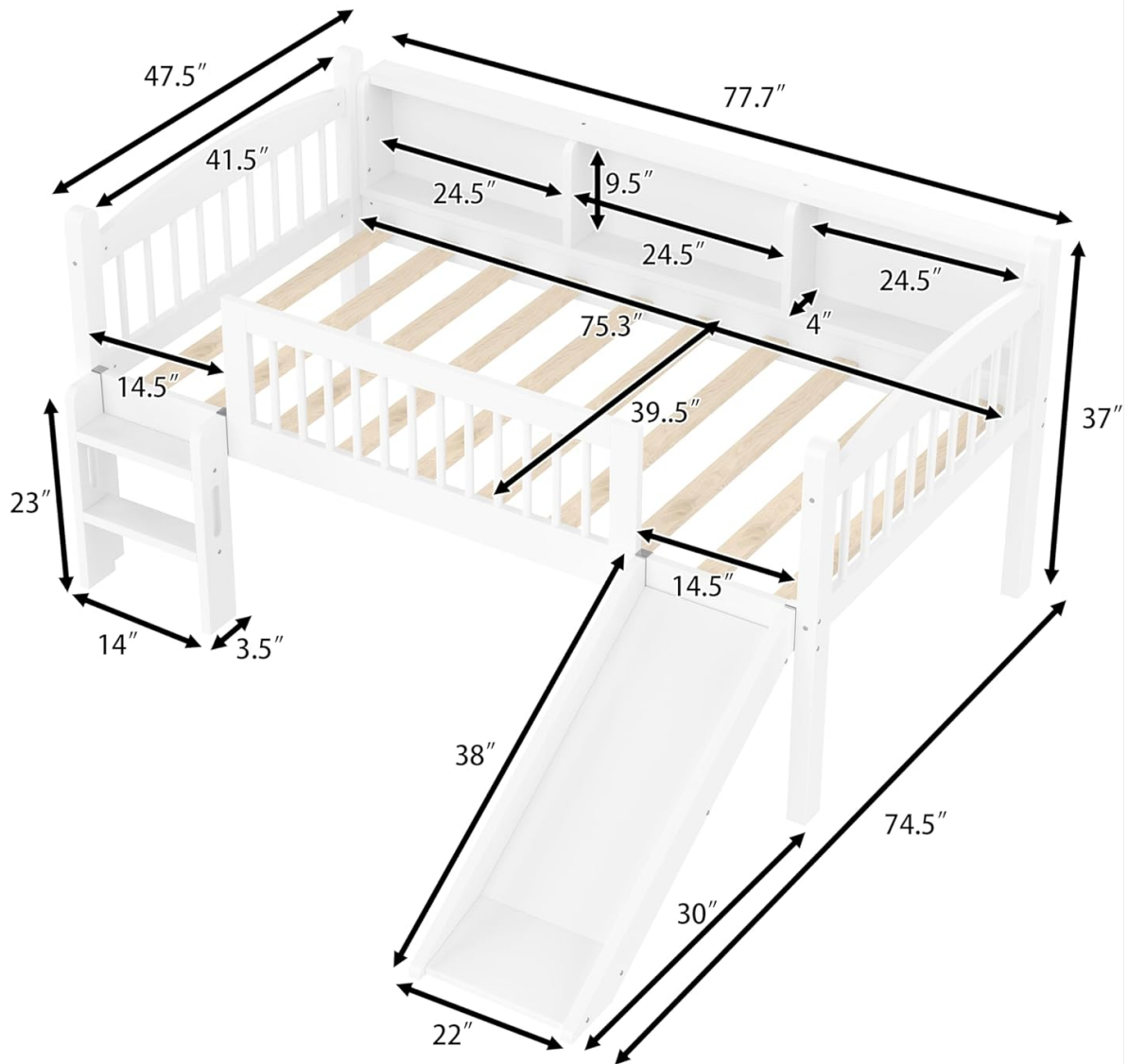
Image: Detailed dimensions of the Bellemave Twin Loft Bed, showing length, width, and height measurements for all components including the bed frame, ladder, and slide.
