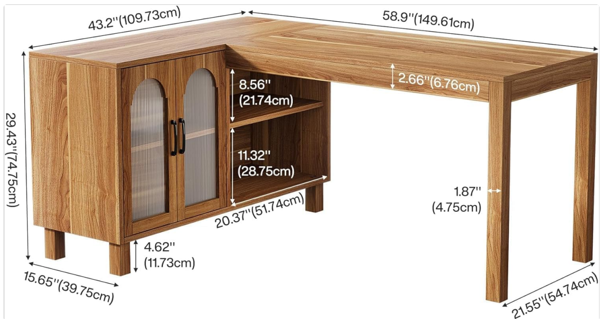
Figure 1: Desk Dimensions. This diagram illustrates the overall dimensions of the L-shaped desk, including the length, width, and height of the main desk surface and the integrated storage unit.
