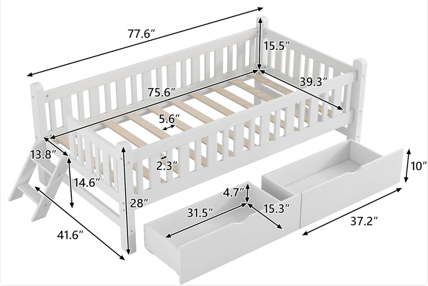
Image 2.1: General view of the Bellemave Twin Platform Bed with guardrails and two storage drawers.
