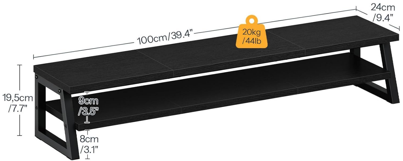
Image: Detailed dimensions and weight capacity of the HOOBRO EBB122CJ01 monitor stand.
