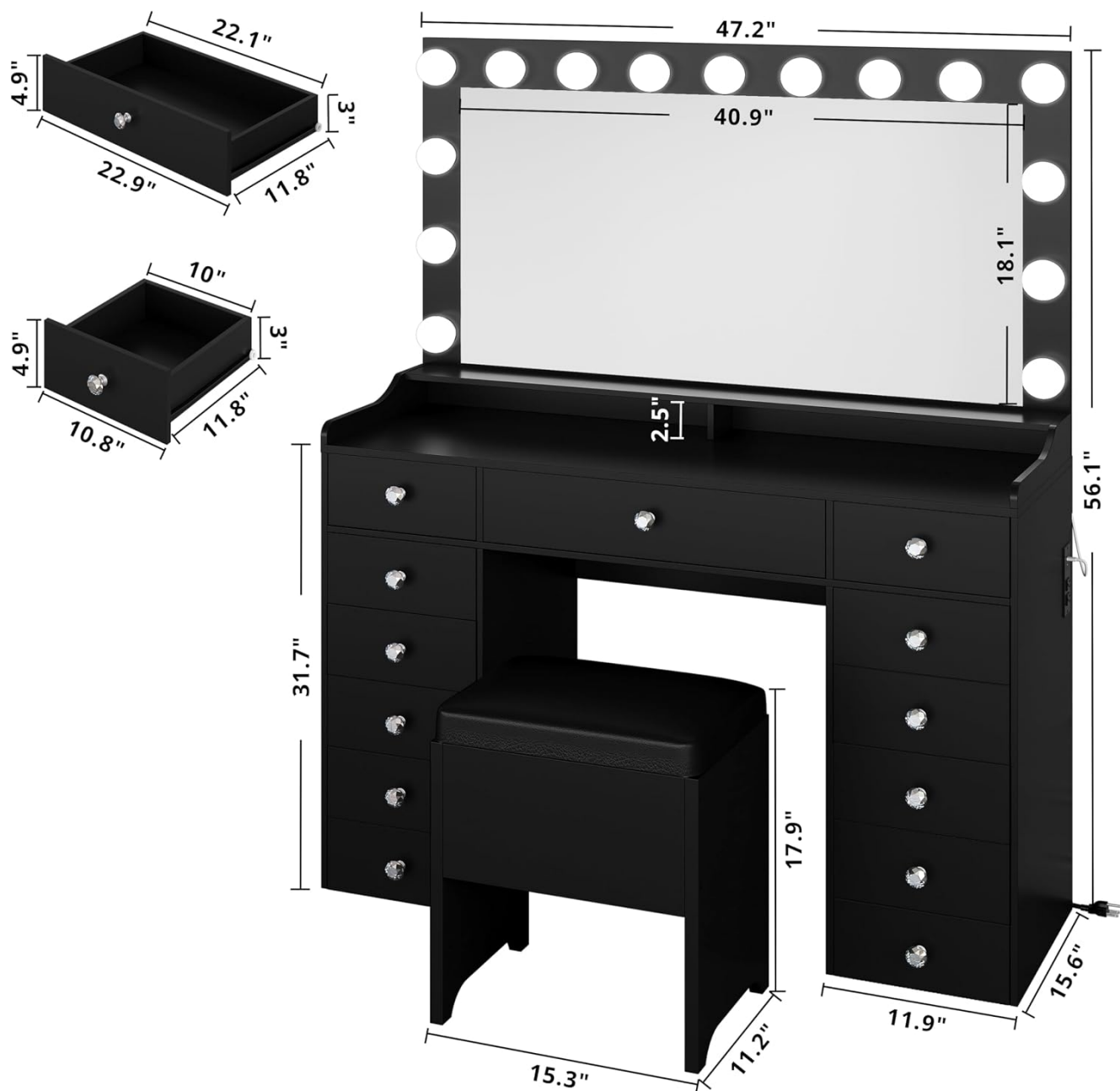
Figure 3.1: Overall dimensions of the IRONCK Vanity Desk.
