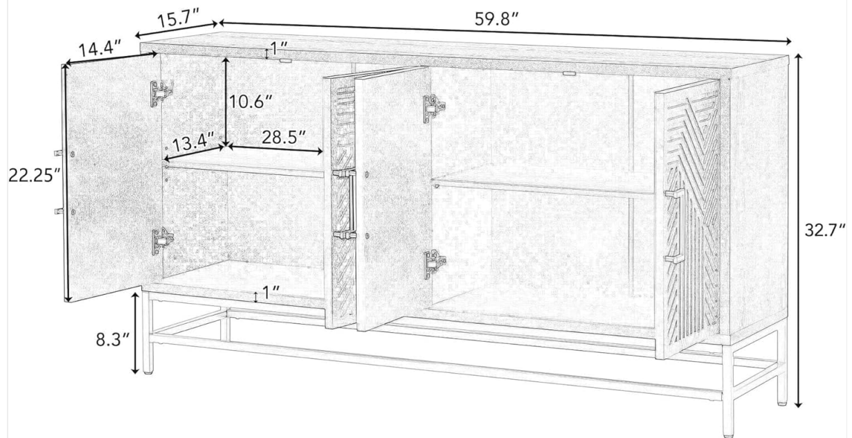
Detailed dimensions of the Virubi Sideboard Buffet Cabinet. All measurements are in inches.
