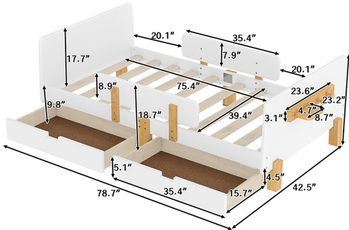
Image 2.1: Detail of the safety guardrail and bed frame construction.
