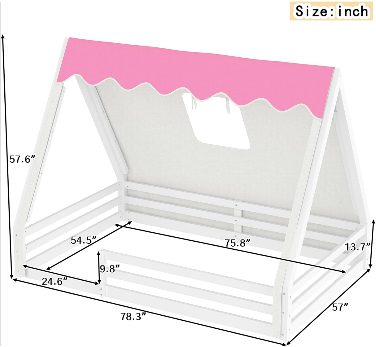
Image 7.1: Detailed dimensions of the SOFTSEA Full Size House Bed, including length, width, and height measurements.
