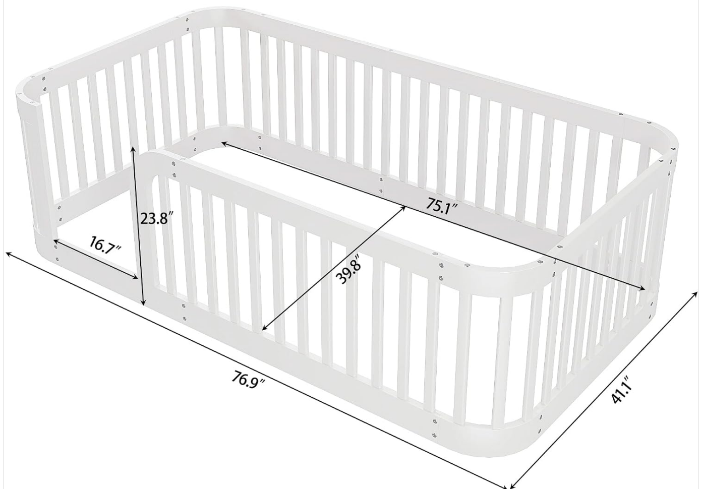
Image 4.1: A diagram illustrating the key dimensions of the assembled bed frame, useful for planning placement.
