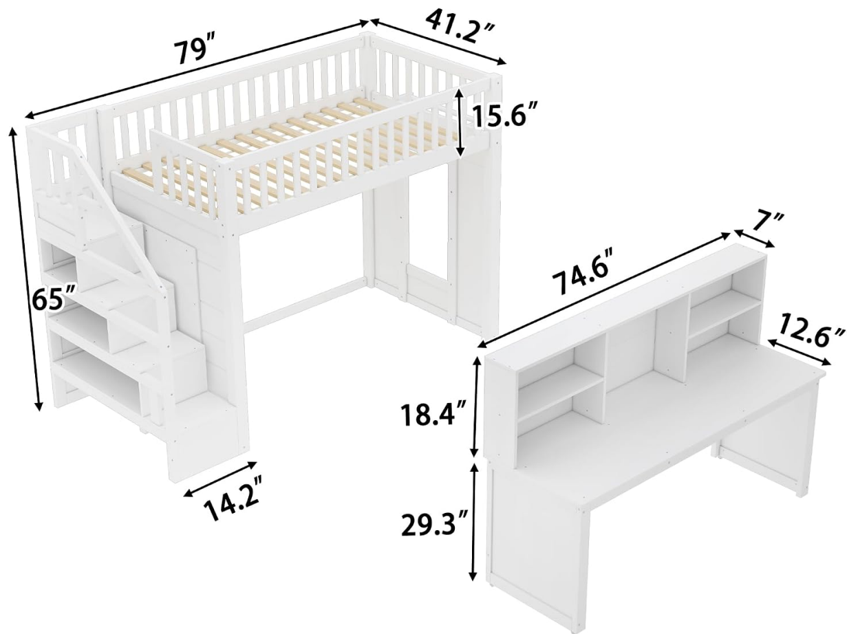
Image 4.1: Detailed dimensions of the loft bed, desk, and stairs in inches.
