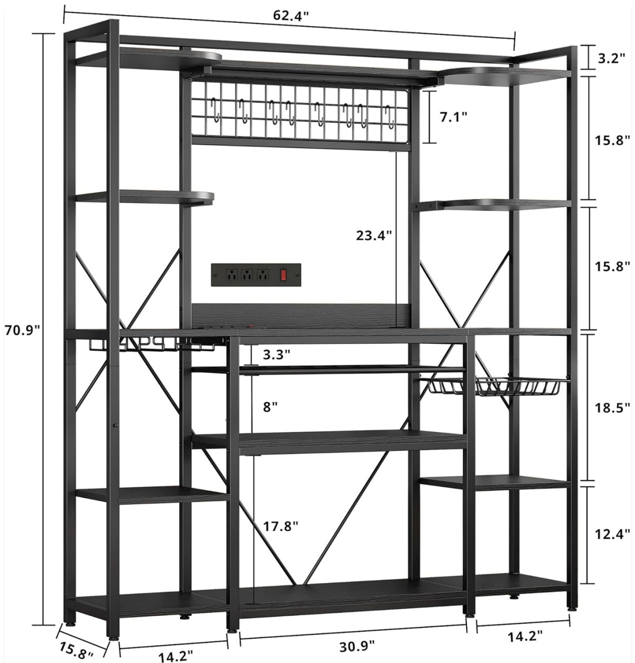
Image 4.1: Dimensional overview of the bakers rack, useful for planning placement and assembly.
