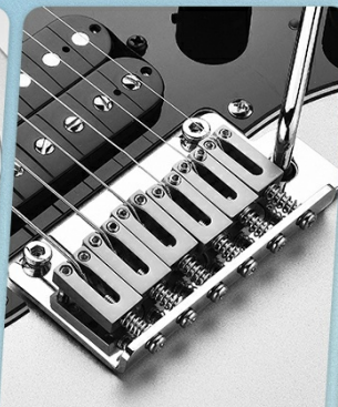
Tremolo Bridge
