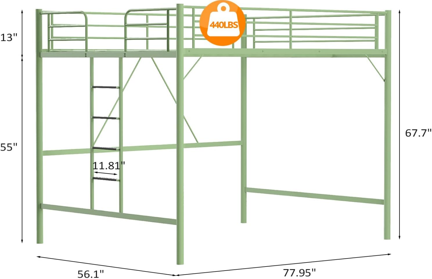
Image: Diagram illustrating the key dimensions of the VINGLI Full Loft Bed, including length, width, height, and under-bed clearance.
