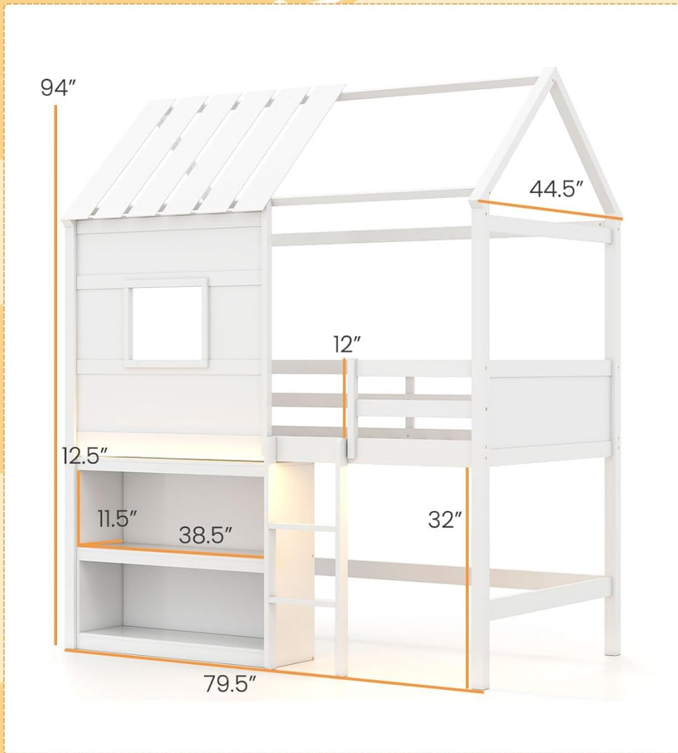
Figure 3: Detailed dimensions of the Giantex Twin Size Loft Bed, including height, length, width, and bookshelf measurements.
