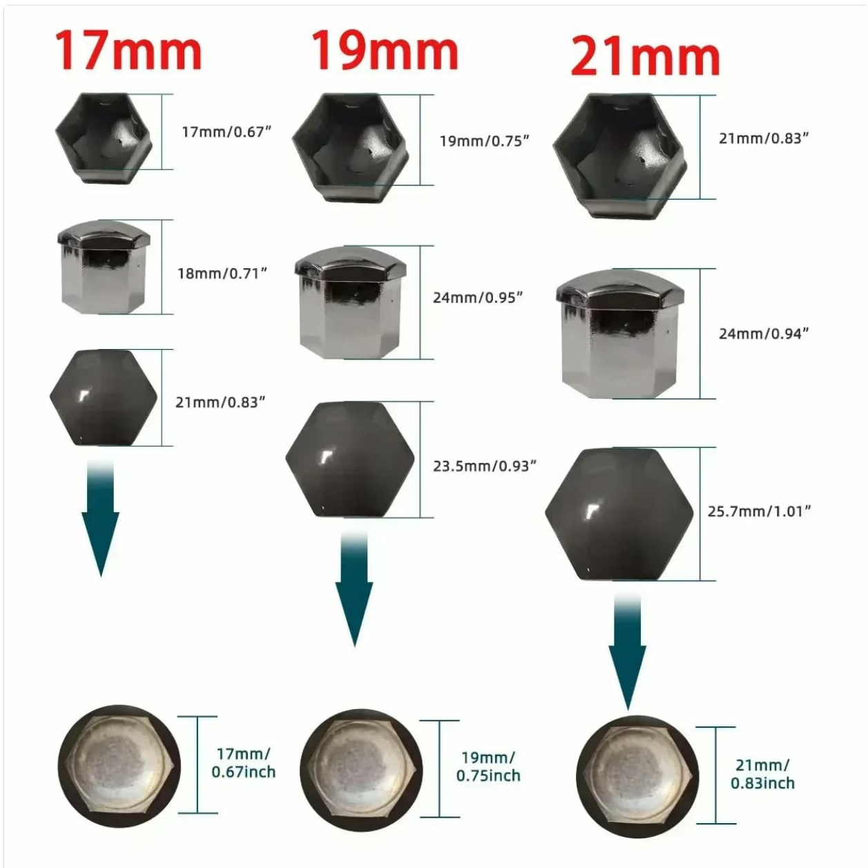
Image: Detailed dimensions for 17mm, 19mm, and 21mm wheel nut covers, illustrating their fitment.
