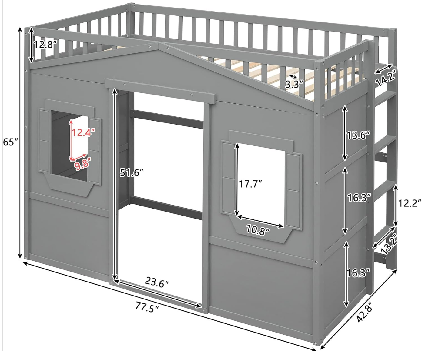
Image: Detailed dimensions of the Bellemave Twin Size Loft Bed, showing length, width, and height measurements in inches. The image highlights the 77.5" length, 42.8" width, and 65" height, along with specific measurements for the windows, door, and ladder steps.
