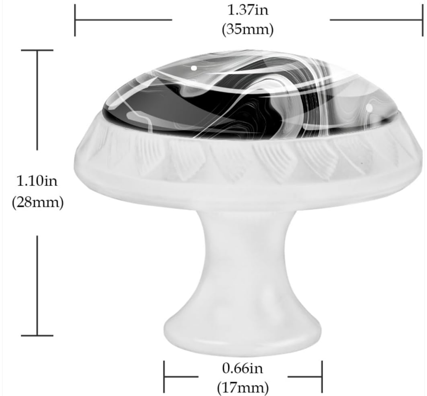
Image 3.1: Detailed dimensions of the drawer knob, including top diameter, base diameter, and height.
