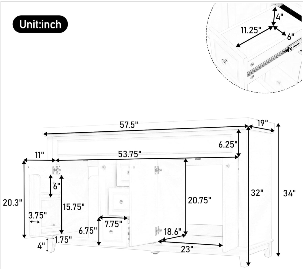
Figure 4: Internal Storage View
