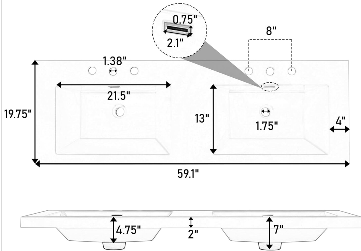
Figure 7: Sink Dimensions
