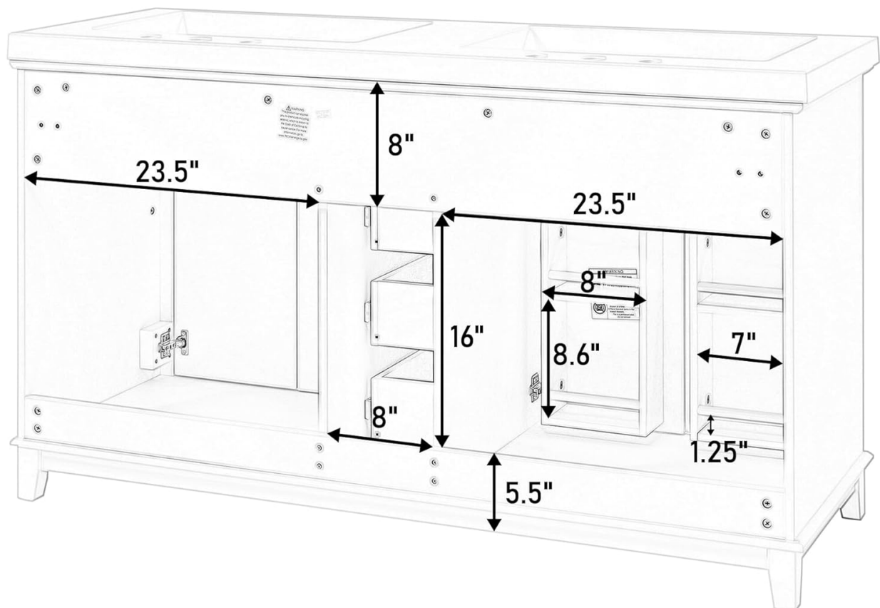
Figure 1: Front View Dimensions
