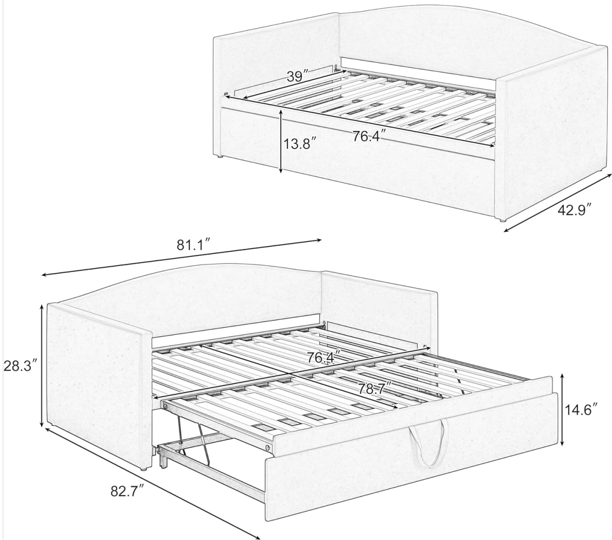
Image 7.1: Dimensional drawing of the daybed, showing measurements for both the compact twin and extended king configurations.
