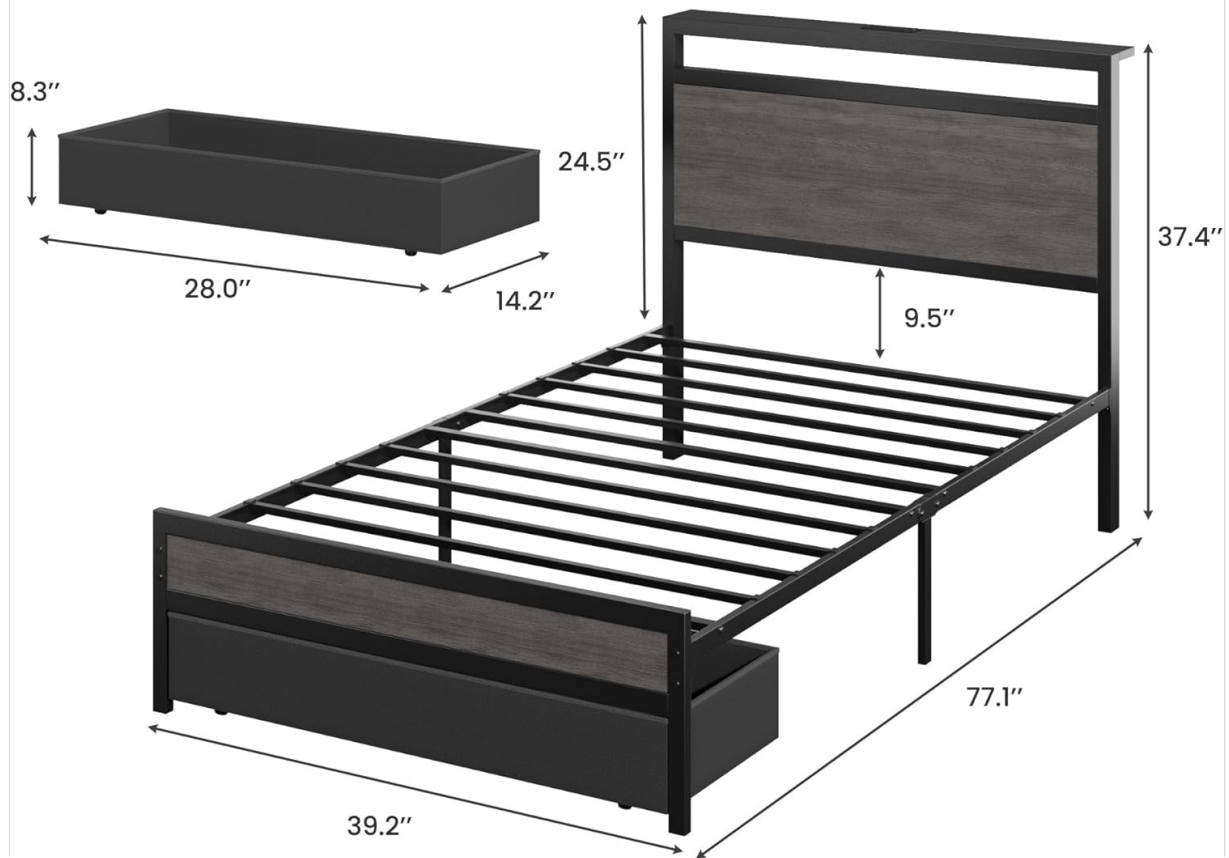
Figure 1: Overall dimensions and main components of the Fluest Twin Bed Frame. Dimensions are 77.1"L x 39.2"W x 37.4"H.
