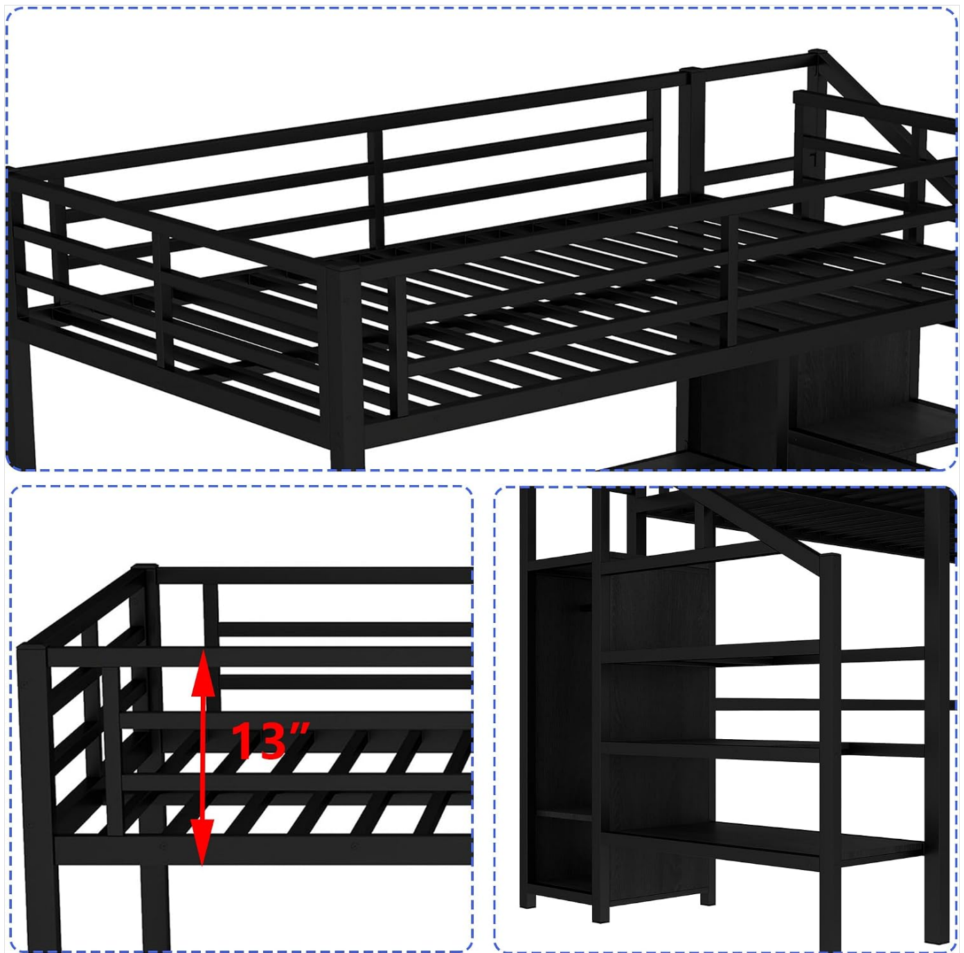
Image: Detailed view of the loft bed frame, illustrating the guardrail height and the robust metal slat support system for mattress stability.
