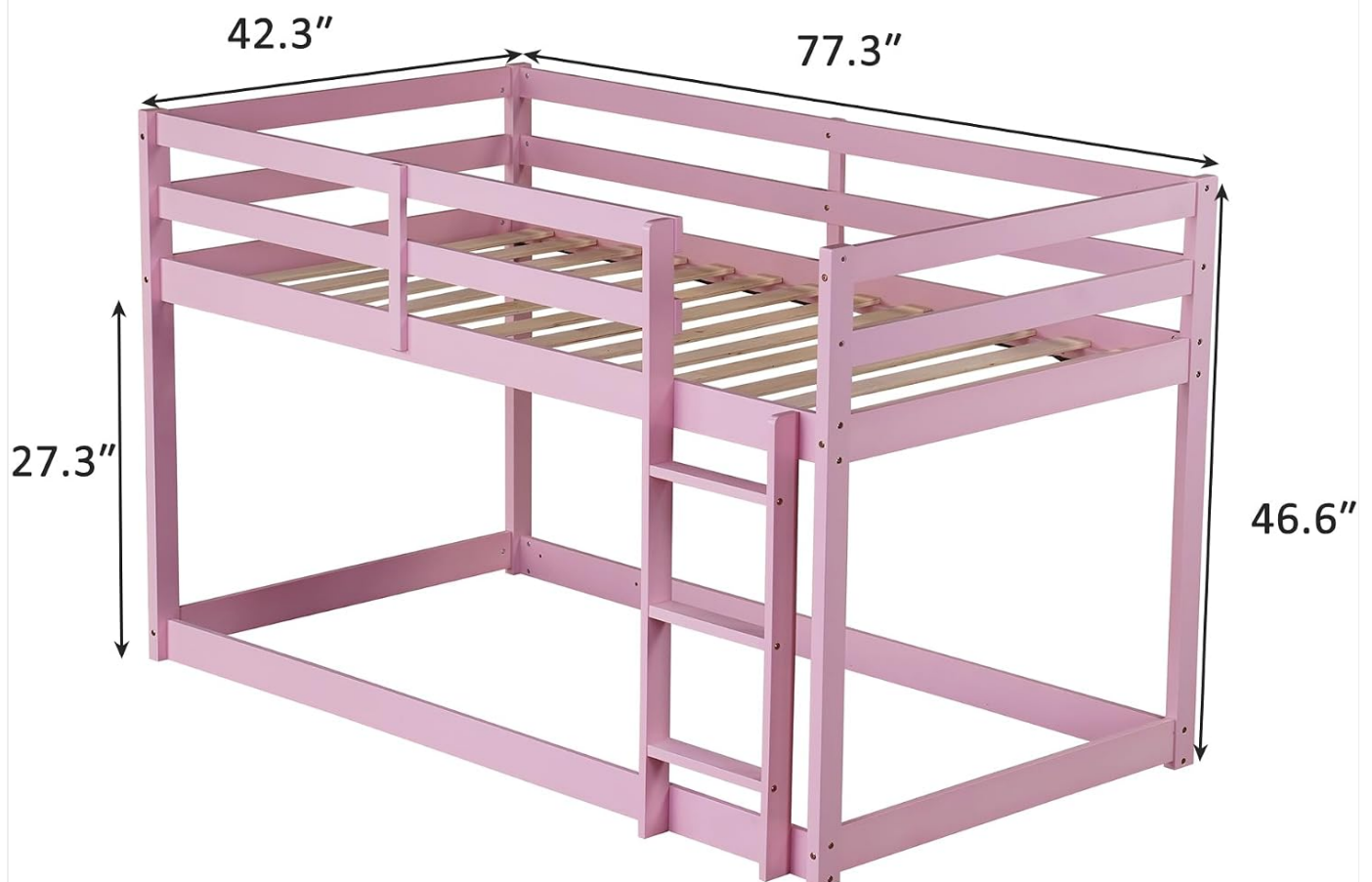
Figure 3: Product dimensions for planning placement.
