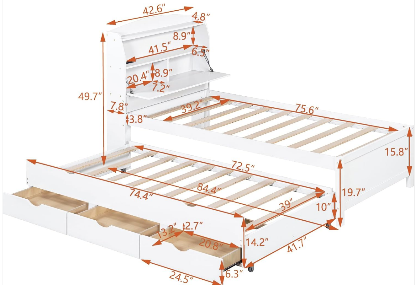
Image: Dimensional diagram for the Twin size bed, illustrating overall measurements and specific component sizes.
