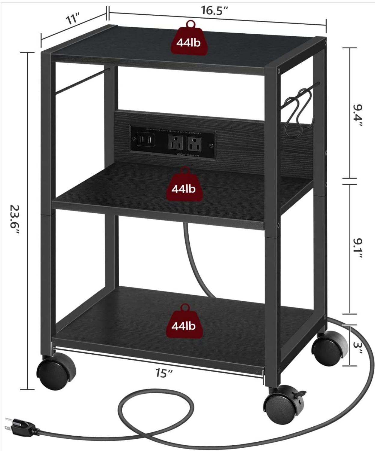
Image: Detailed dimensions and weight capacity for the MAHANCRIIS Industrial Printer Cart. The cart measures 16.5 inches long, 11 inches wide, and 23.6 inches high. Each of its three shelves can support up to 44 pounds.
