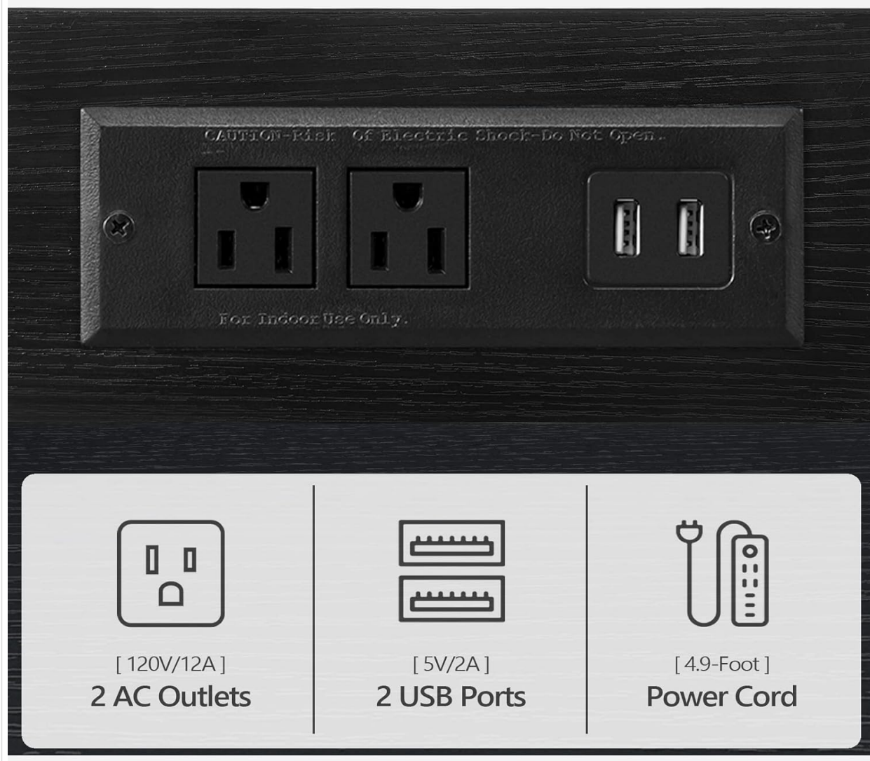
Image: Close-up of the power strip on the MAHANCRIIS Industrial Printer Cart, showing 2 AC outlets (120V/12A), 2 USB ports (5V/2A), and a 4.9-foot power cord.
