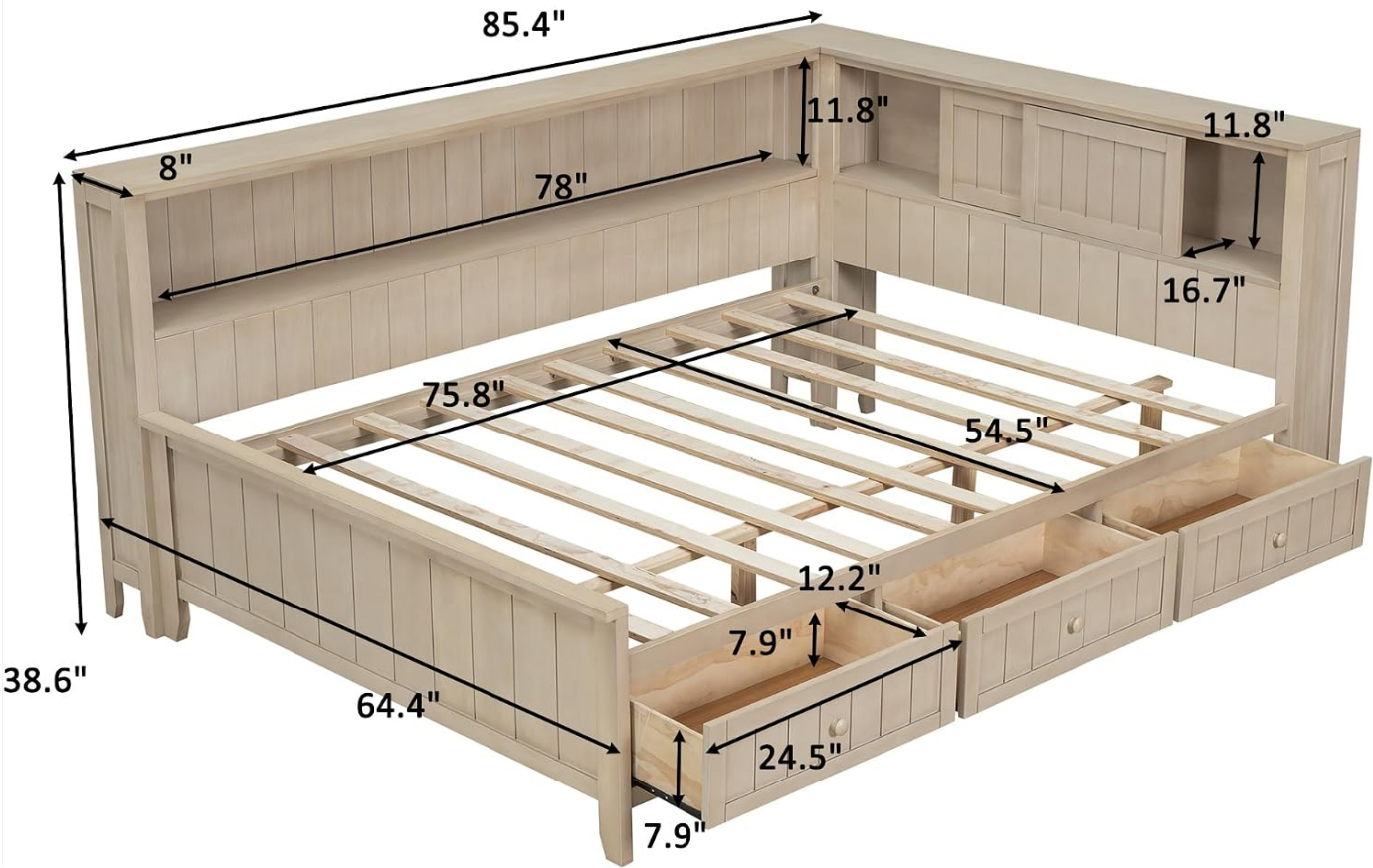
Image 6: Detailed diagram showing the dimensions of the THINK 30 Full Size Wooden Daybed.
