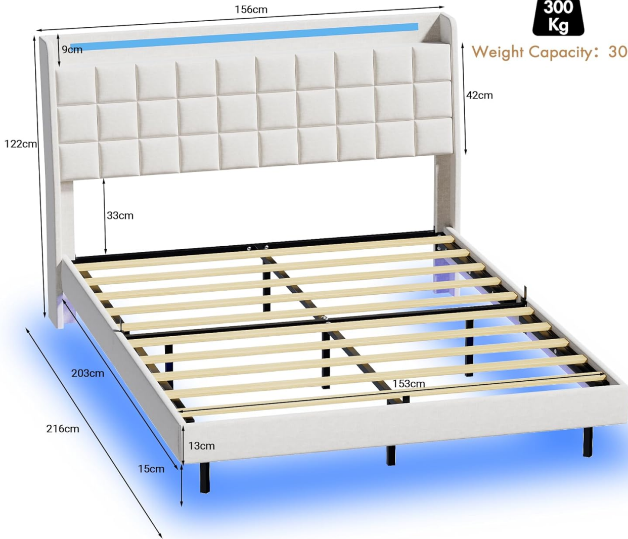
Figure 7.1: Dimensional overview of the Advwin Queen Floating Bed Frame.
