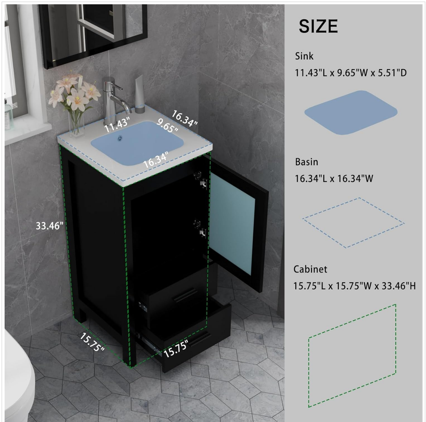
Figure 3.1: Detailed Product Dimensions
