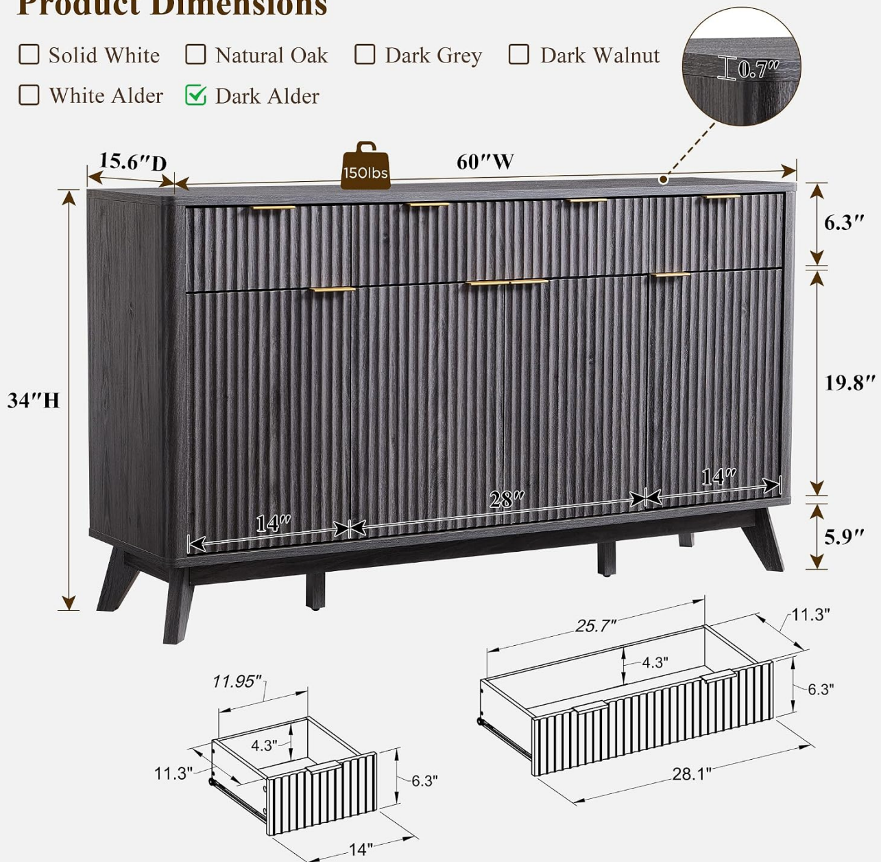
Image 4.1: Detailed dimensions of the cabinet, including width, height, depth, and drawer sizes.
