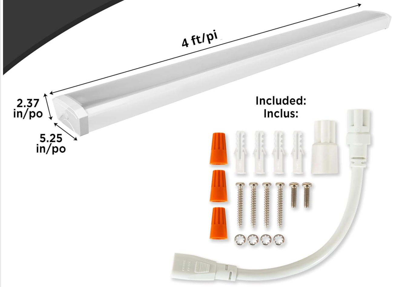
Image: The Luminus 4-ft LED Wrap Light showing its dimensions and the included accessories: wire nuts, screws, anchors, and a connector cable.
