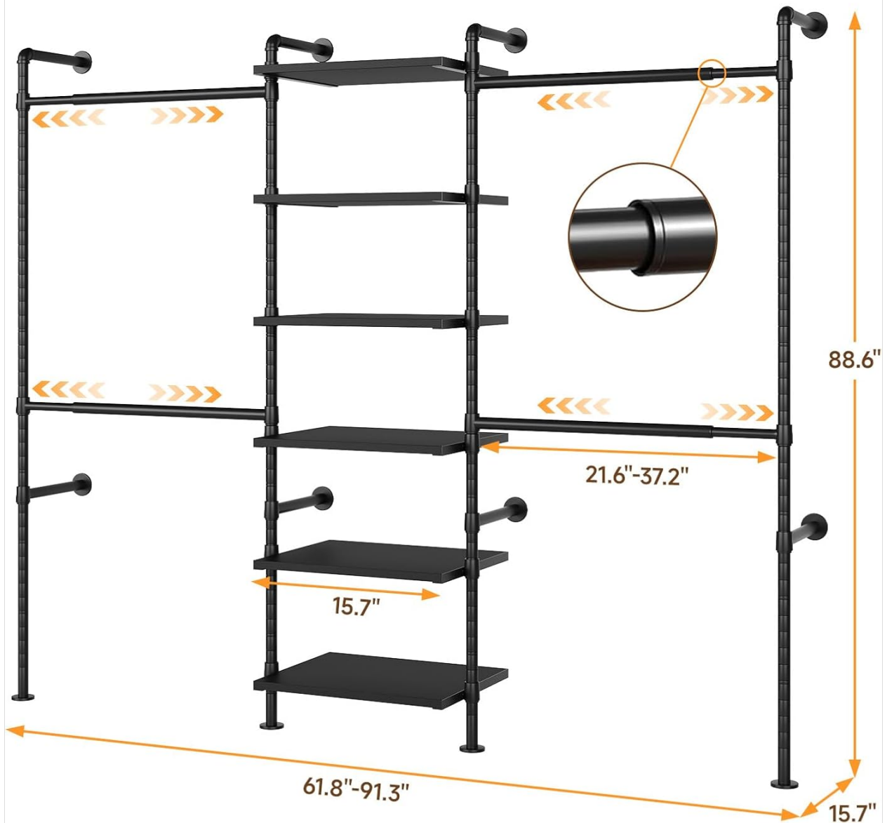
Image 4.3: Dimensional diagram of the closet system, indicating a weight capacity of 1050 lbs and an assembly space requirement of at least 7'6" in height.
