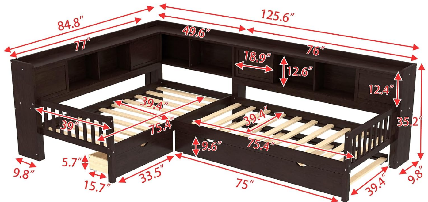
Figure 1: Overall Product Dimensions (Unit: Inches)
