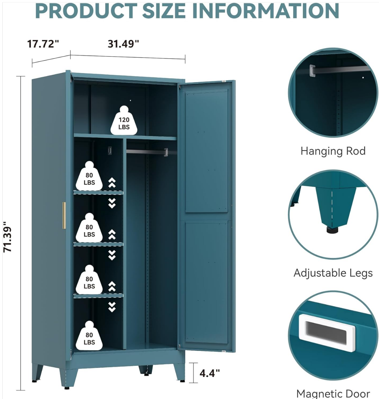
Image 4.1: Overview of product dimensions (17.72"D x 31.49"W x 71.39"H) and key features such as the hanging rod, adjustable legs, and magnetic door closure. Note the weight capacities for shelves (80 lbs each) and the top shelf (120 lbs).
