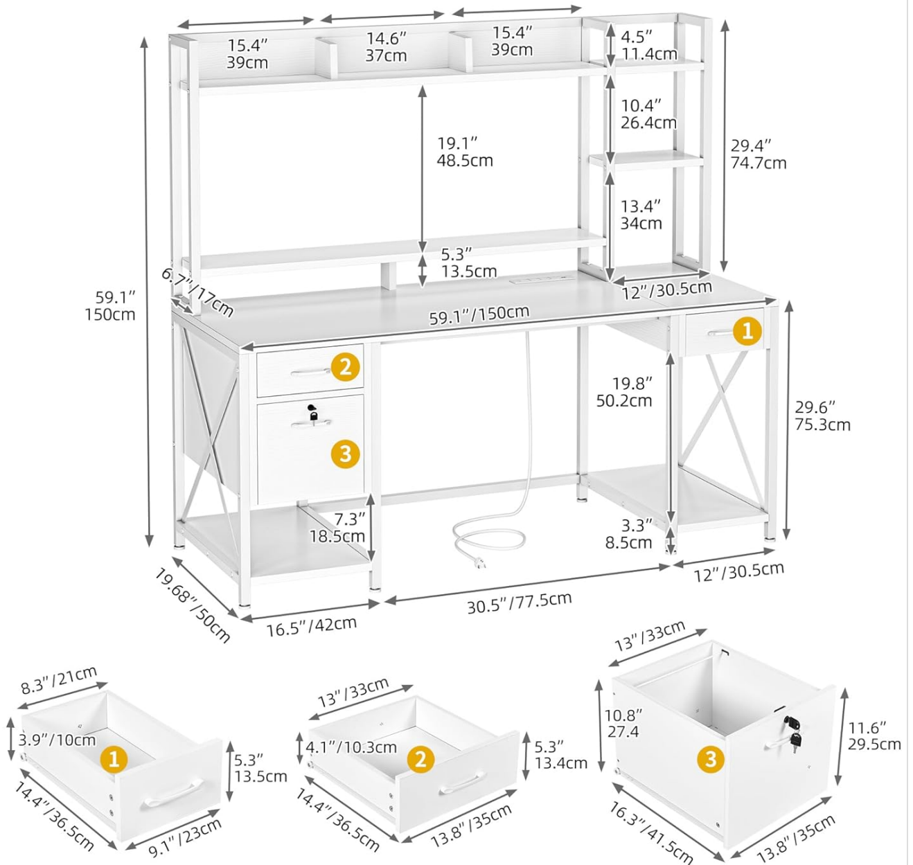
Image: A diagram illustrating the precise dimensions of the desk, hutch, and drawers.
