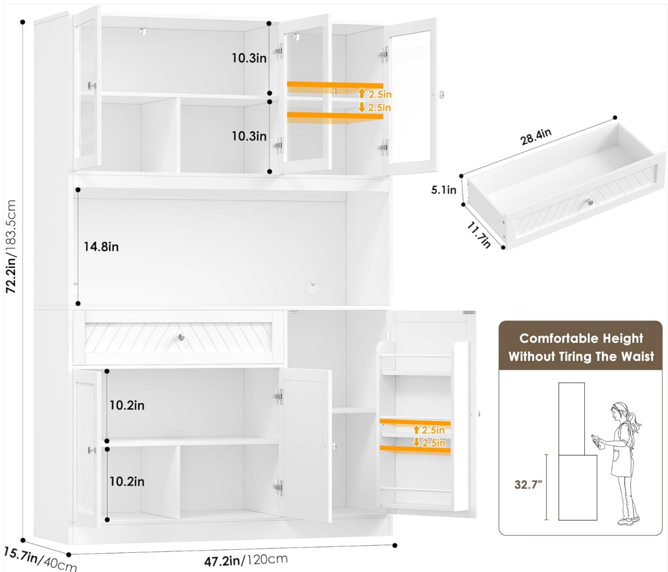
Figure 1: Detailed dimensions and internal layout of the BOTLOG kitchen pantry cabinet, illustrating shelf spacing and overall size.
