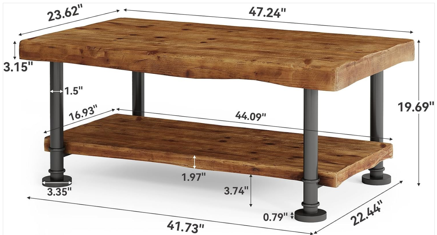
Figure 7.1: Detailed dimensions of the coffee table.
