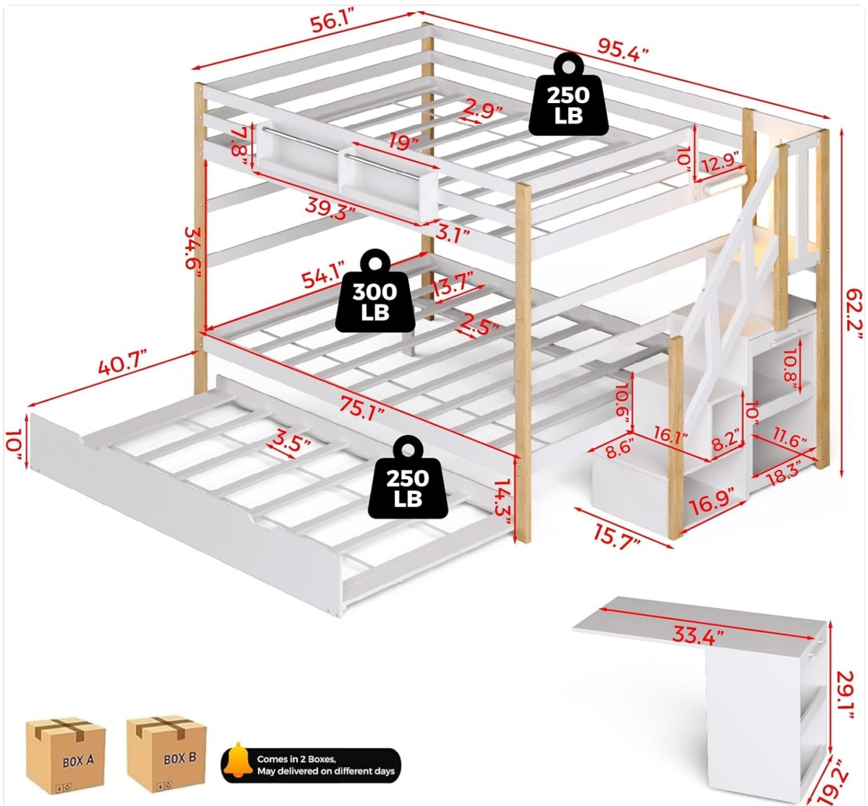
Image 8.1: Detailed diagram illustrating the dimensions of the Full Over Full Bunk Bed with Trundle and Storage Stairs, including length, width, height, and individual component measurements.
