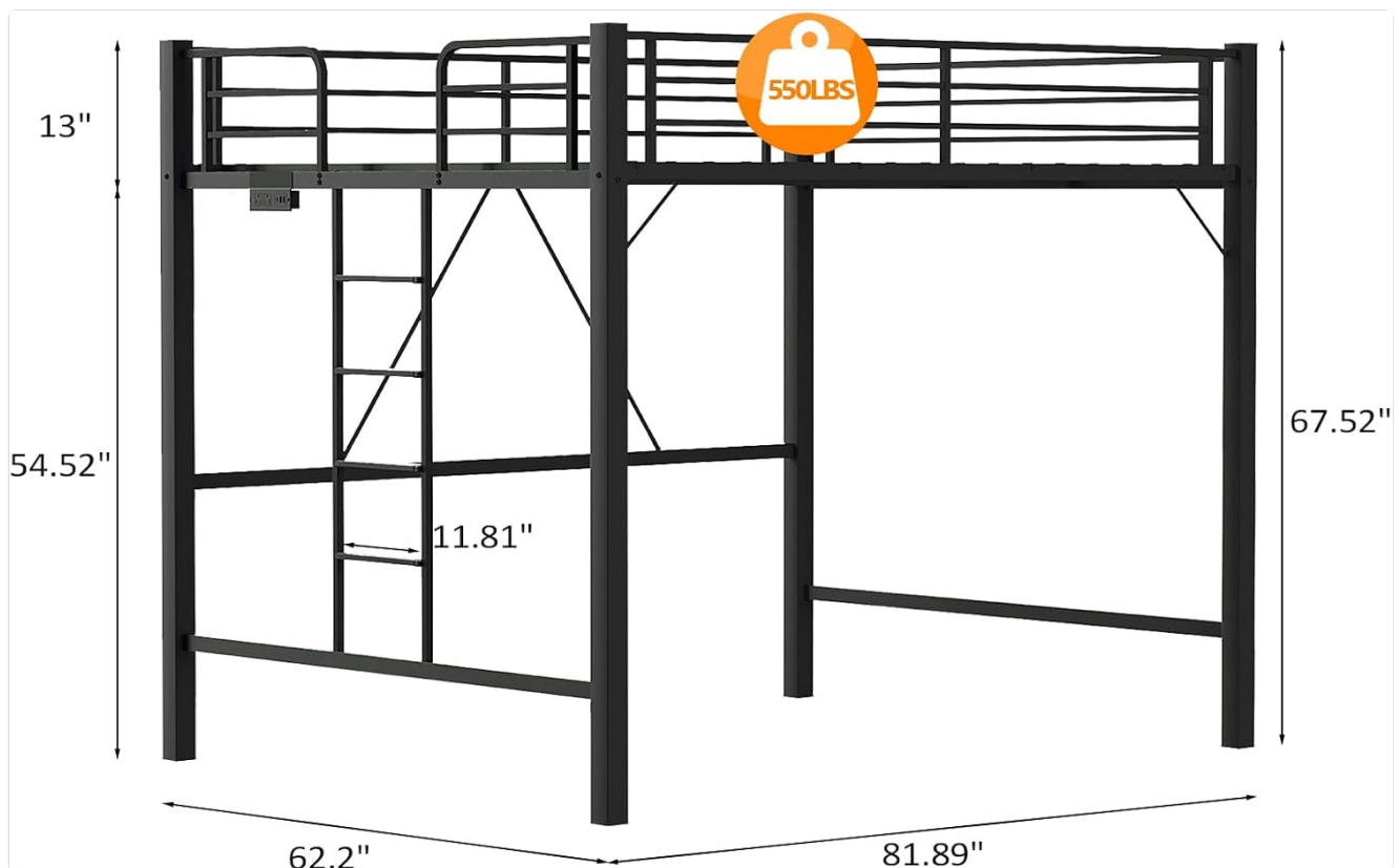
Image 8.1: Key dimensions of the VINGLI Queen Size Loft Bed.
