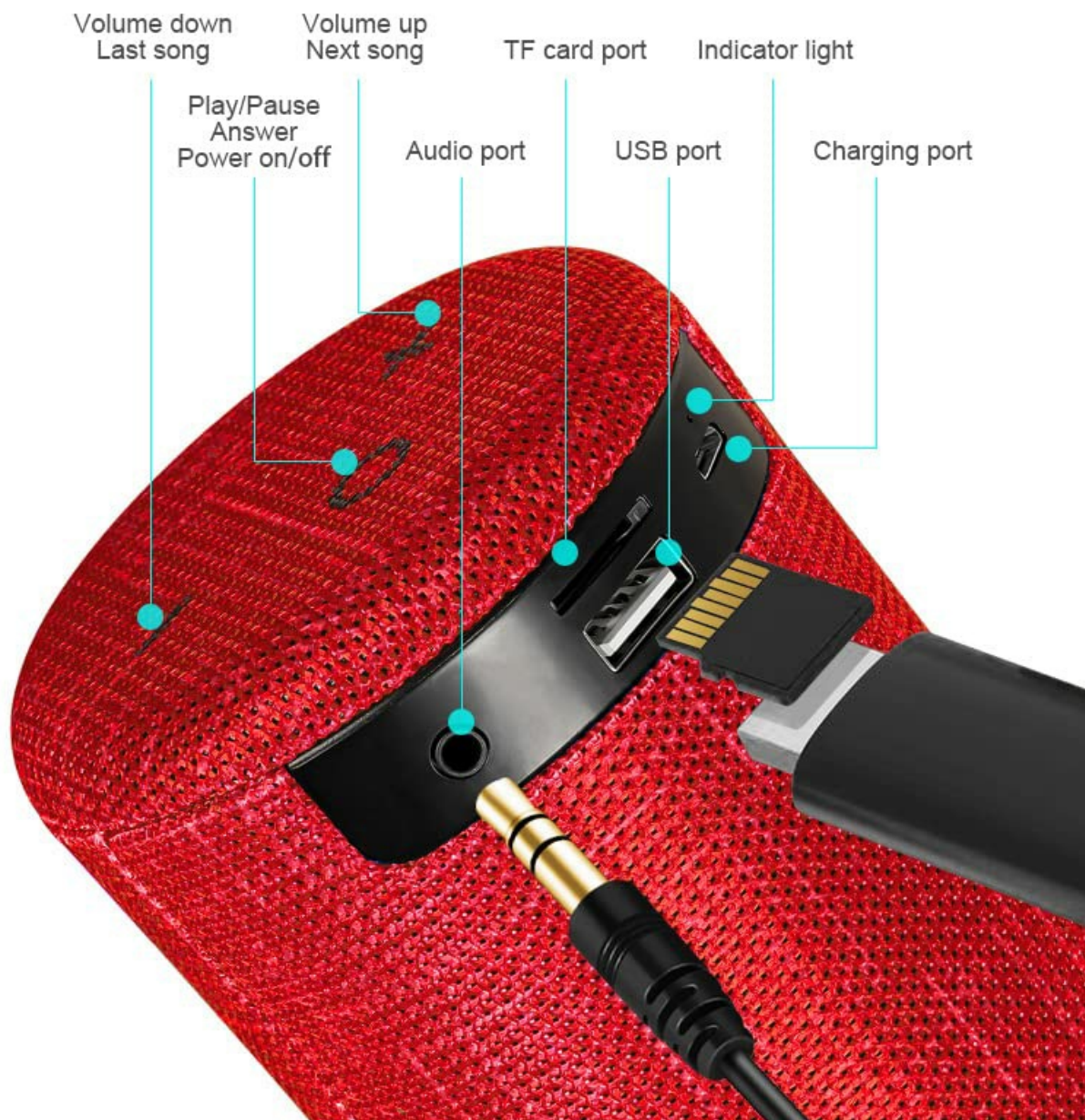
Image 5: Product parameter details for the bwoo BS-52 speaker, including technical specifications.
