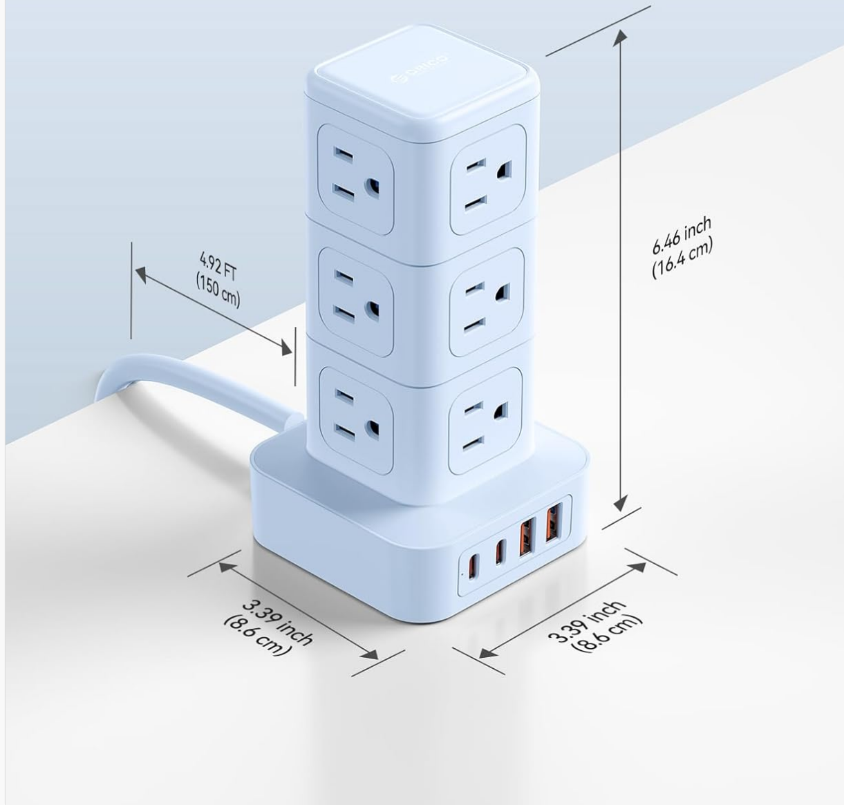
Image: A detailed view of the ORICO Power Strip Tower, illustrating its compact dimensions: 3.39 inches (8.6 cm) in length and width, and 6.46 inches (16.4 cm) in height, with a 4.92 ft (150 cm) cord.
