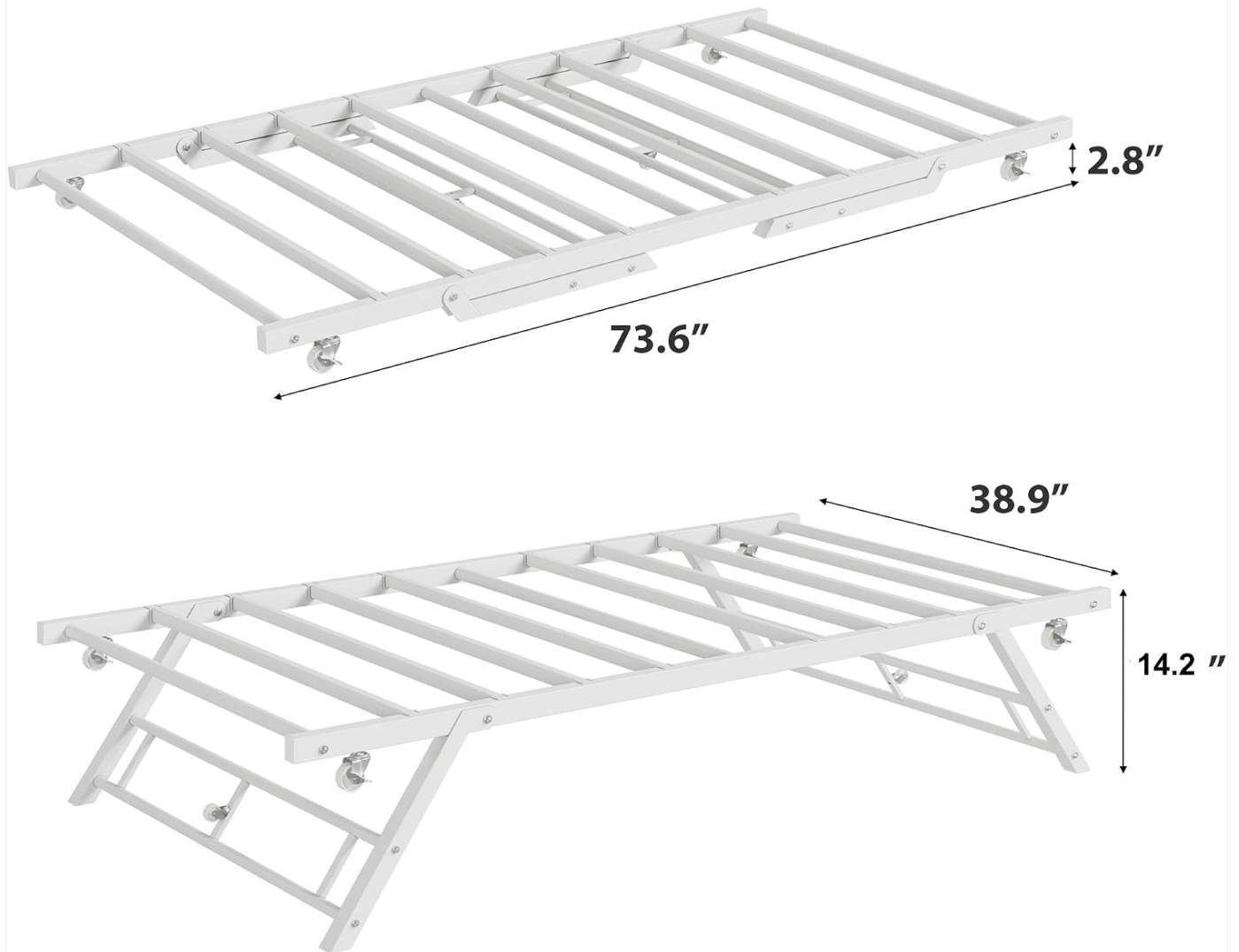
Image: All components of the IDEALHOUSE Twin Pop-Up Trundle Bed frame laid out.
