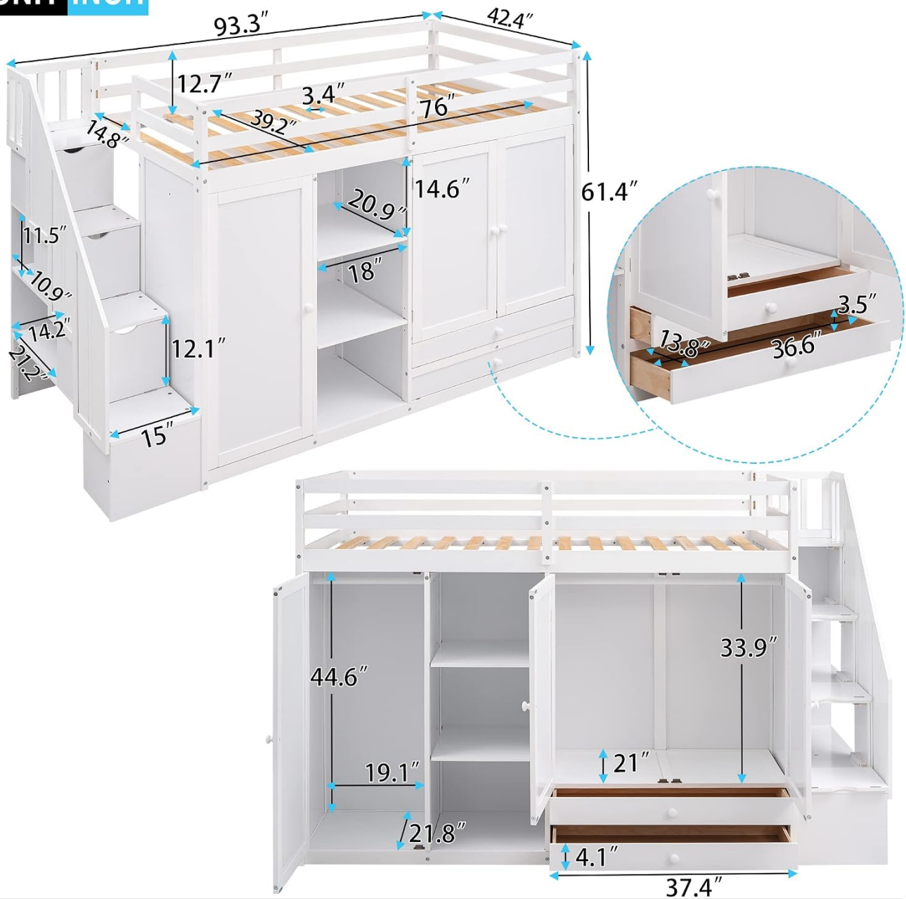
Image: Dimensional overview of the loft bed, useful for planning placement and understanding component sizes during assembly.
